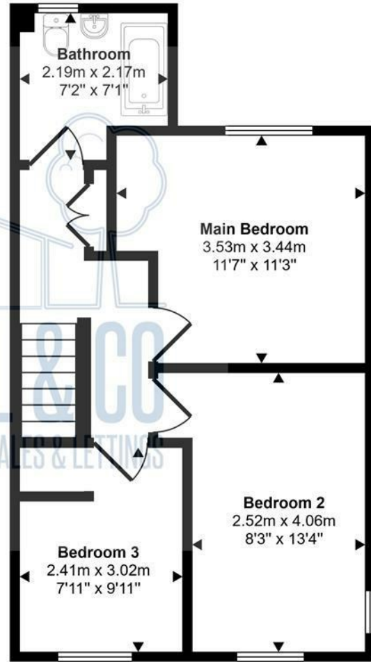
First Floor Approx 43 sq m / 458 sq ft
